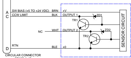
MT2 (CCW) PHOTOELECTRIC SENSOR SUNX PM-L24
