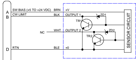
MT1 (CW) PHOTOELECTRIC SENSOR SUNX PM-L24
